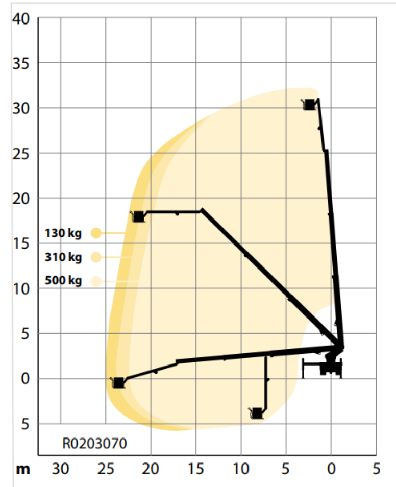
F32TLK outreach diagram (18t)
