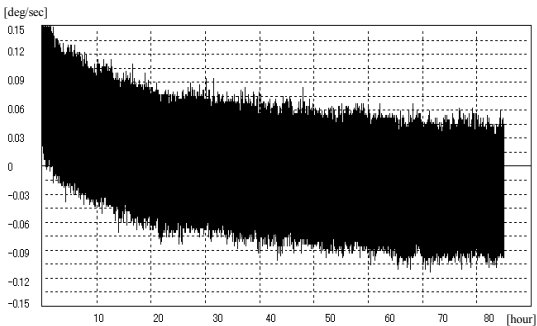
Fig 6 Sensor 2 Y axis rate output
